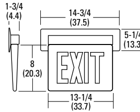
Back Mount (recessed)
