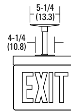
With Pendant Mounting kit (TM mounting only)
