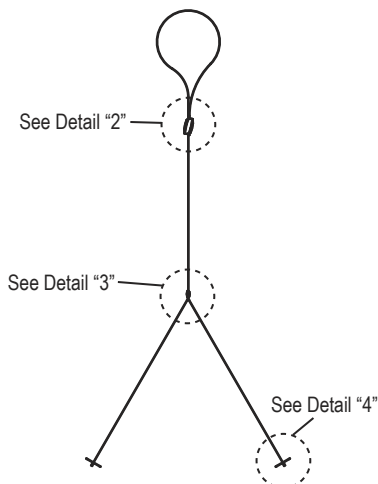
Single Adjustable Loop Y with toggle (MHYTG)
