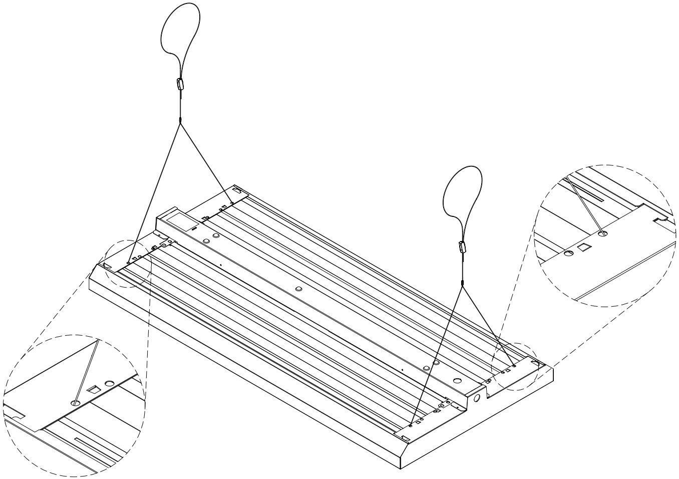
Detail "1" Swedged Connection
