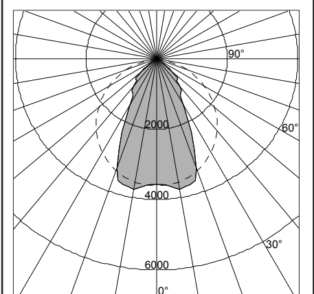
FTT 1 CF40 0U/2D T1X32 Test #T12369_S Fixture Efficiency: 99.8% SC Across: 0.9, SC Along: 1.3
