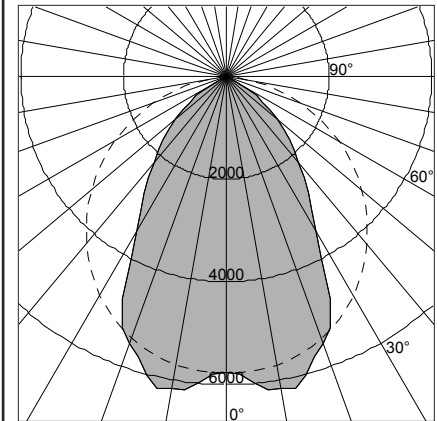
FTT 2 CF40 0U/2D T1X32 Test #T12320_S Fixture Efficiency: 90.8% SC Across: 1.0, SC Along: 1.3
