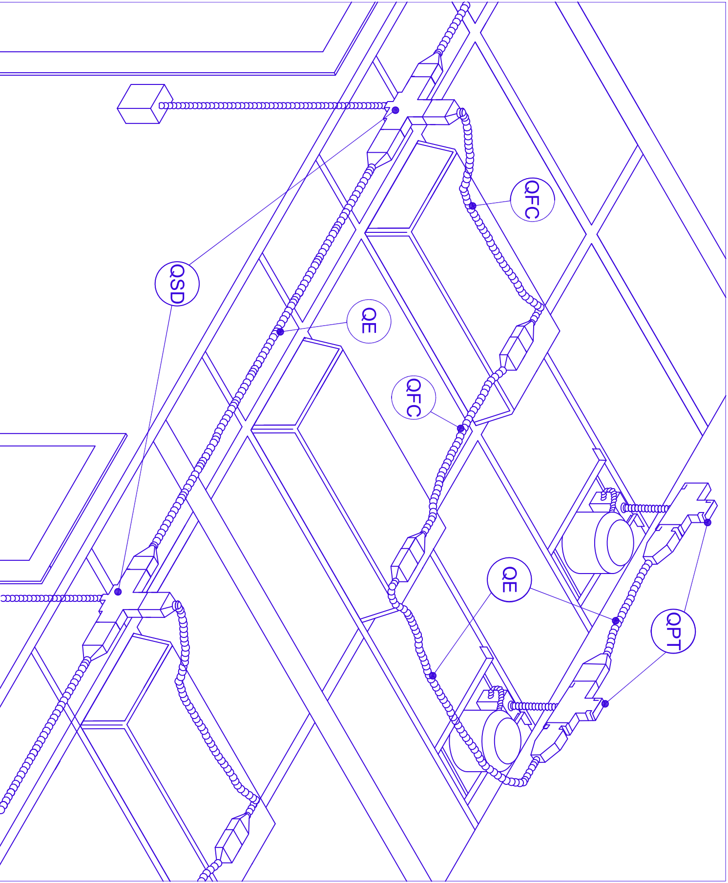
Typical QuickFlex System View
