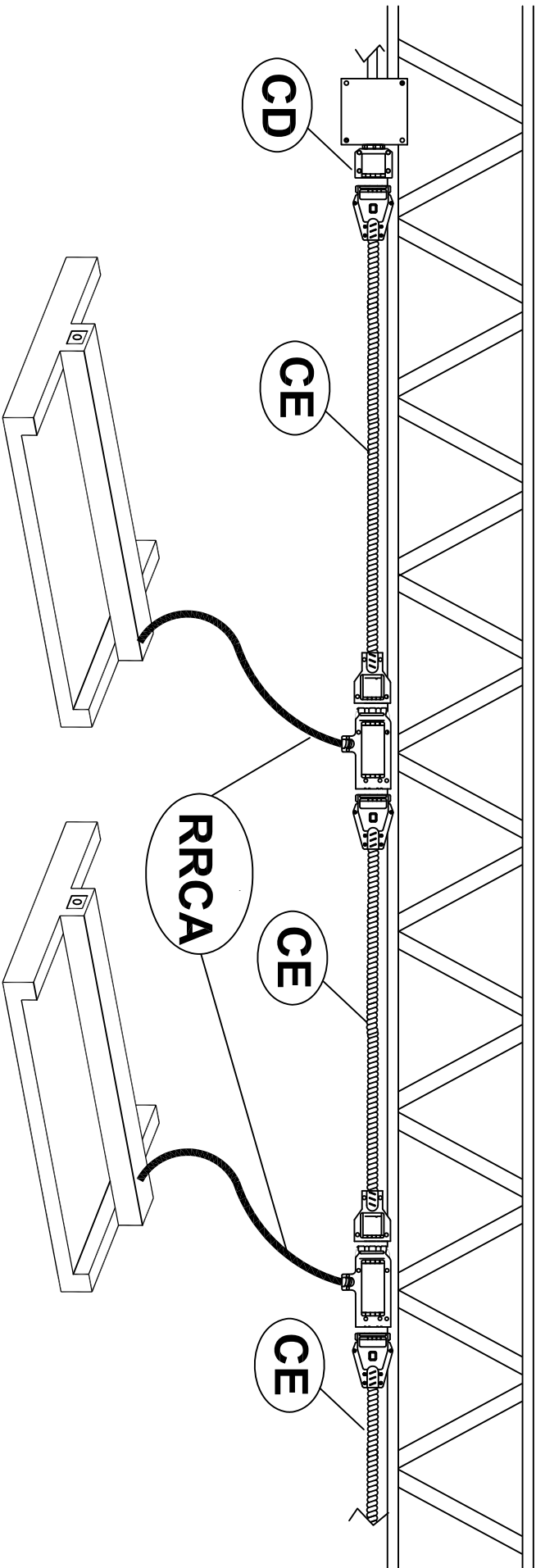
SYSTEM VIEW - REPLACEMENT RELOC CORD ASSEMBLY
