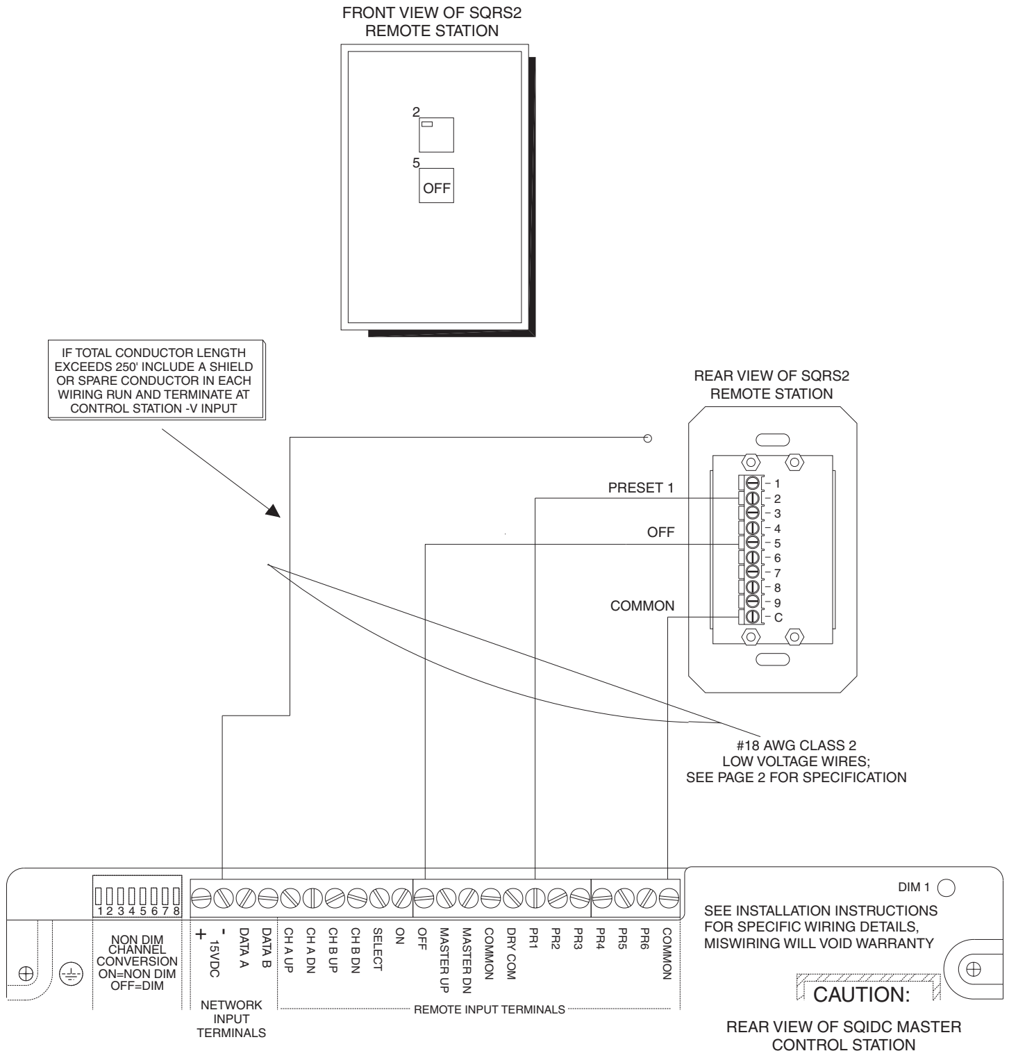
Figure 5 - Sequel IDC Control Station to SQRS2S Remote Control Station Interconnection Wiring Details
