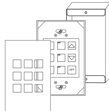
Figure 2 - Exploded View of Remote Station
