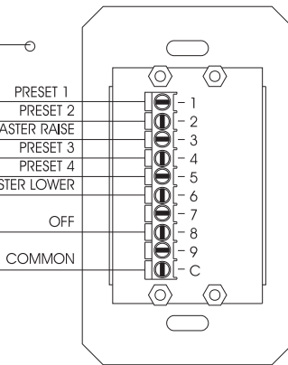
REAR VIEW OF SQRS7 REMOTE STATION
