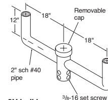
2U bull horn 2" slip fitter BKT-18-PP 2 3/8" tenon BKT-19-PP 4" tenon
