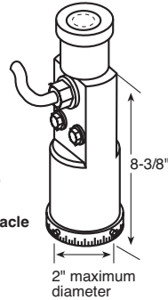
08664-XXX mounting adapter yoke to 2" slip fitter, cast aluminum, painted with photocontrol substitute voltage for "XXX"
