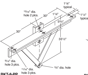
BKT-8-PP 3 light cross-arm 08647 required for middle fixture
