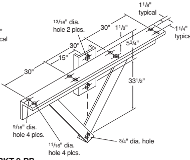
BKT-9-PP 4 light cross-arm
