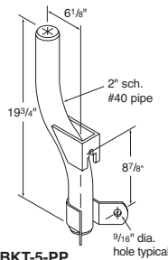
BKT-5-PP wood pole bracket 2" slip fitter
