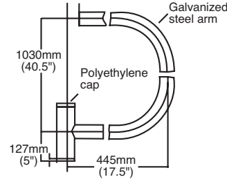
ARM160/170 Shepards Crook
