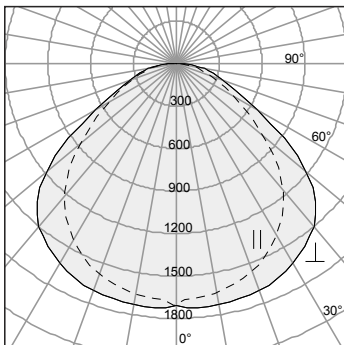
MBH24 2 32 A12 Test #LTL7424M Fixture Efficiency: 81.7% SC Across: 1.4, SC Along: 1.2
