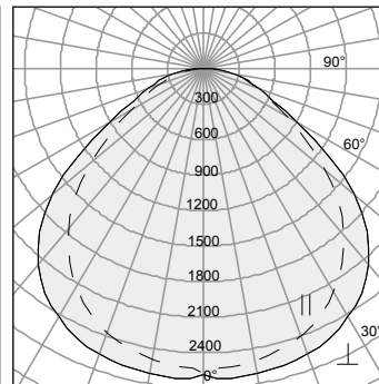
MBH24 3 32 A12 Test #LTL7421M Fixture Efficiency: 80.2% SC Across: 1.4, SC Along: 1.2
