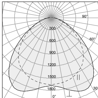
MBH24 2 32 S1X12 A12 Test #ALP200290M Fixture Efficiency: 85.1% SC Across: 1.6, SC Along: 1.3
